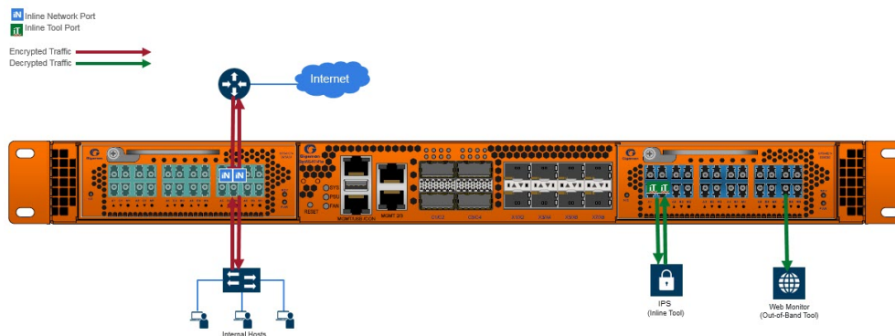
Figure 45 GigaVUE Modules: GigaSMART and Inline Bypass
