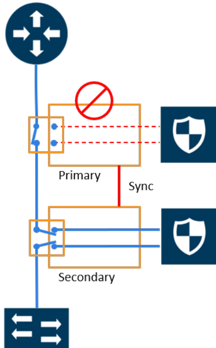
Figure 22 Traffic Flows Through Node with Secondary Role after Primary is Lost
