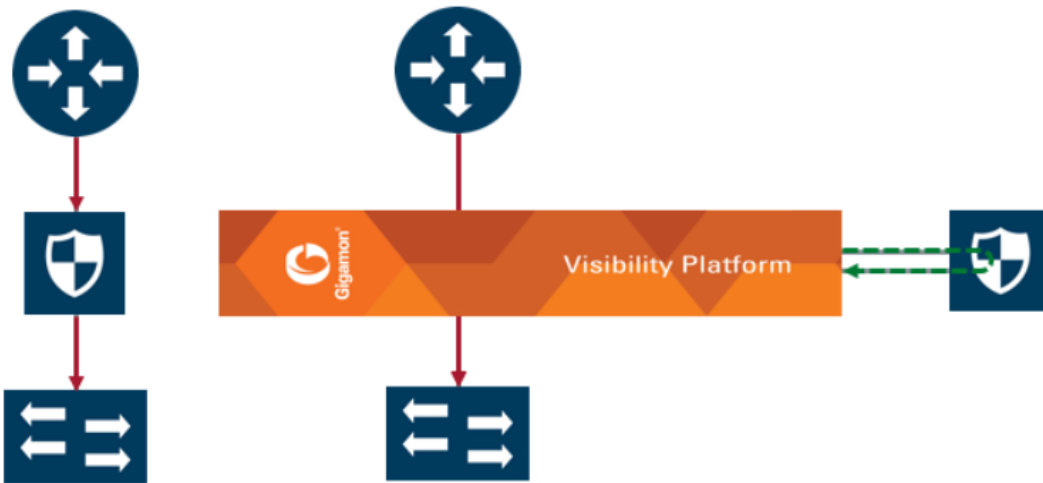
Figure 40 Simple Inline Tool Arrangement
