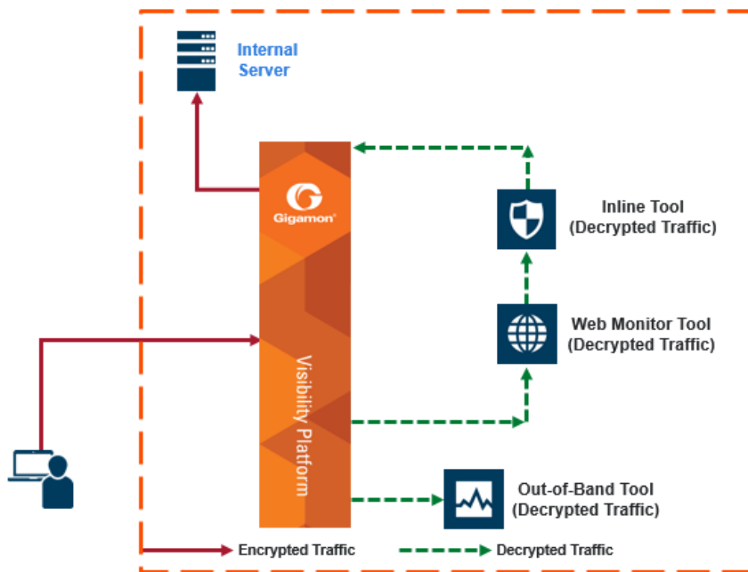
Figure 35 Inbound Deployment of Inline TLS/SSL Decryption
