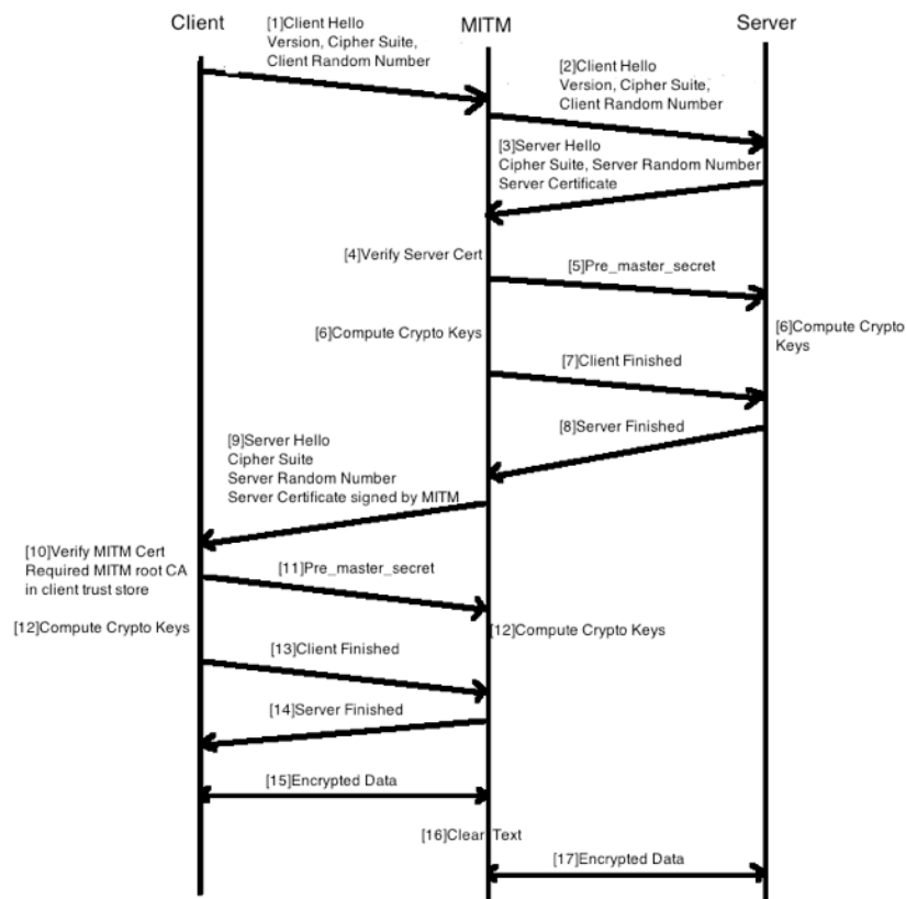
Figure 34 Man-in-the-Middle TLS/SSL Handshake
