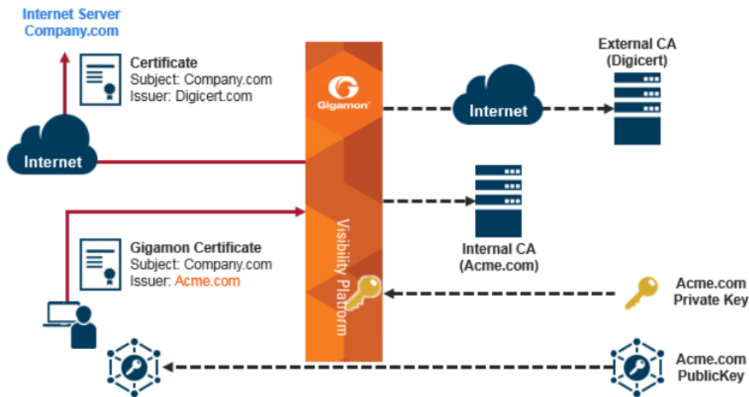
Figure 36 Outbound Deployment of Inline TLS/SSL Decryption
