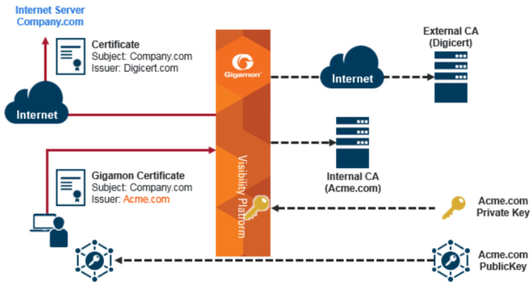
Figure 44 Outbound Deployment of Inline TLS/SSL Decryption
