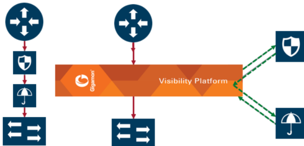
Figure 42 Serial Inline Tool Arrangement
