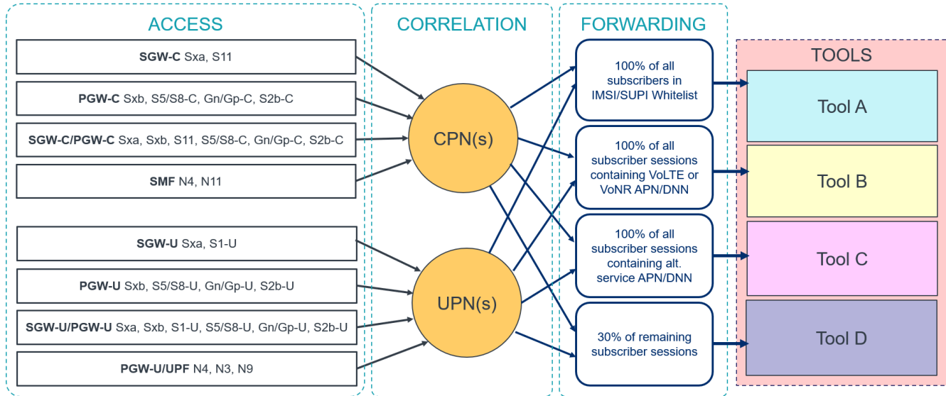
Figure 22 CUPS Traffic Visibility Solution
