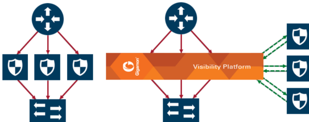
Figure 41 Multiple Inline Tool Arrangement
