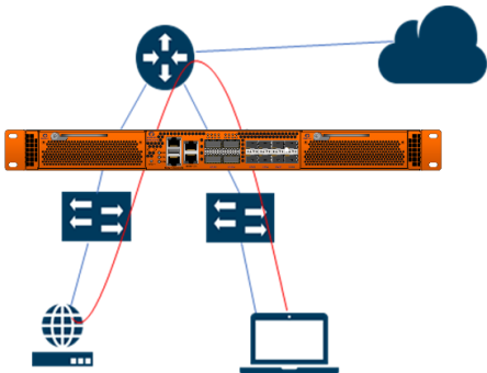
Figure 39 Inline TLS/SSL Inline Network Group Configuration
