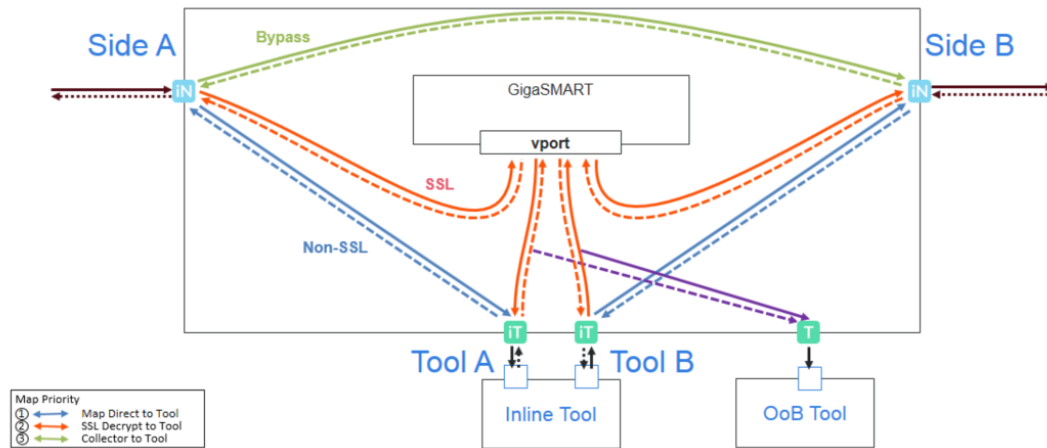
Figure 46 Packet Flow for Inline SSL Decryption
