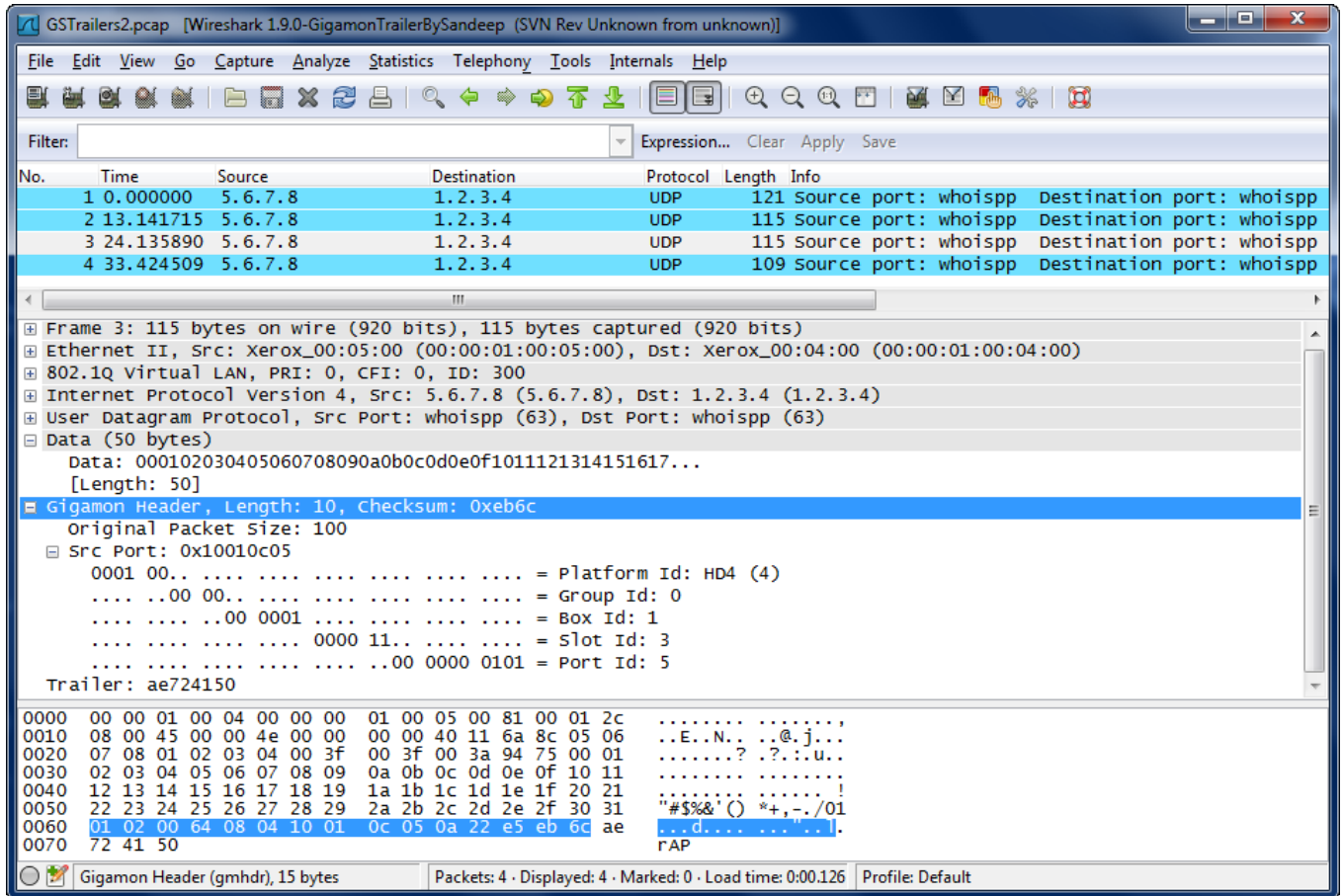
Figure 153 Wireshark Decode of GigaSMART Trailer
